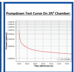
PUMPDOWN TEST CURVES
